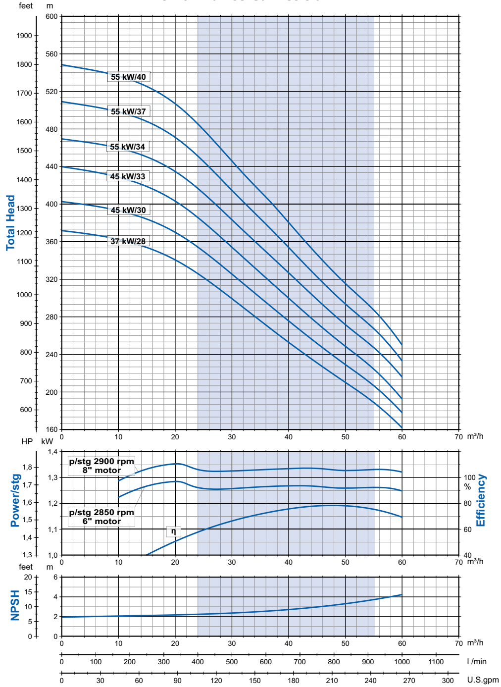
Performance Curves 50 Hz
