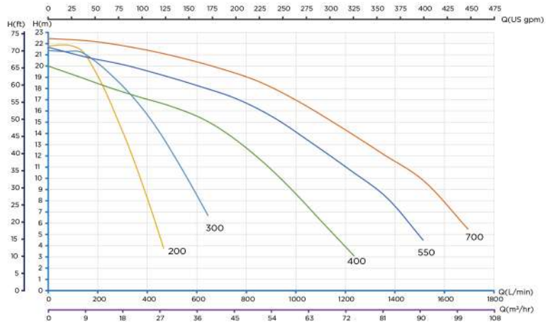
Hydrostar MK4 Performance Chart
