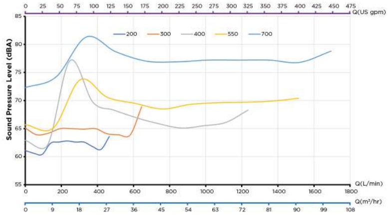
Hydrostar MK4 Sound Levels
